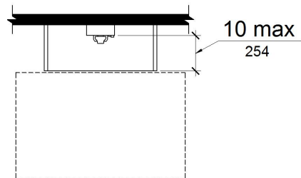
Figure 11B-704.2.1.1 Parallel Approach to Telephone
